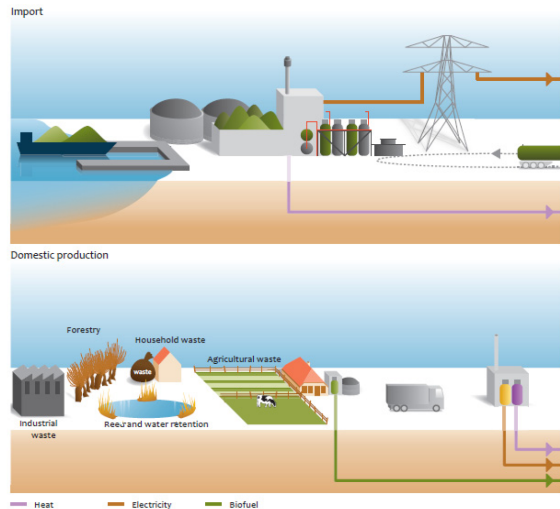
Figure C 8: Energy production
